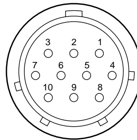
DC PARALLEL INPUT
